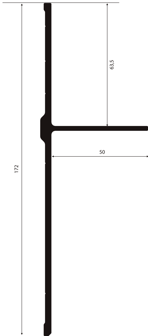
NI-682 1,981 Kg/m
