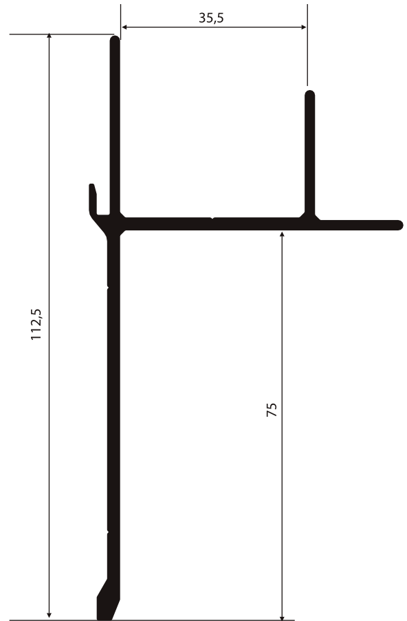
NI-420 1,264 Kg/m
