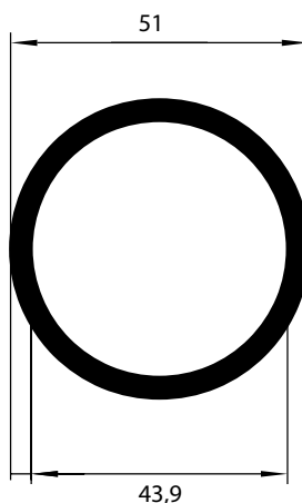
NI-2202 1,434 Kg/m
