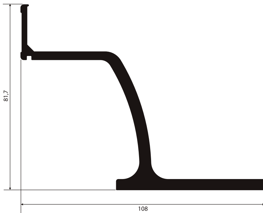
NI-937 2,296 Kg/m
