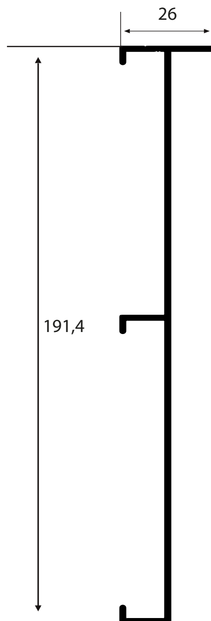
NI-2052 1,097 Kg/m
