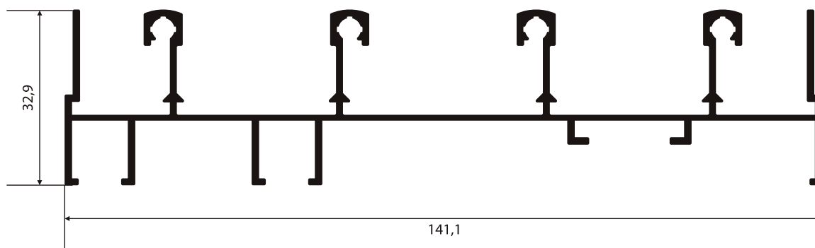
SU-121 1,415 Kg/m
