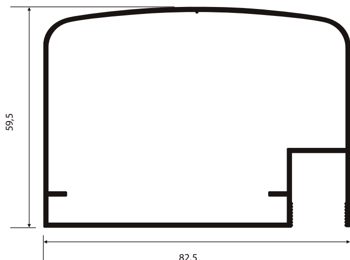
NI-409 1,131 Kg/m
