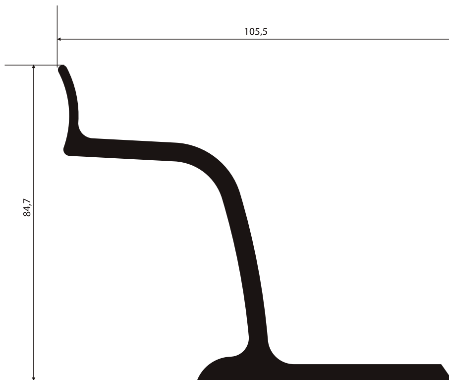
NI-938 2,415 Kg/m
