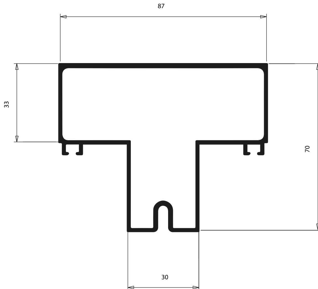
FA-400 1,453 Kg/m
