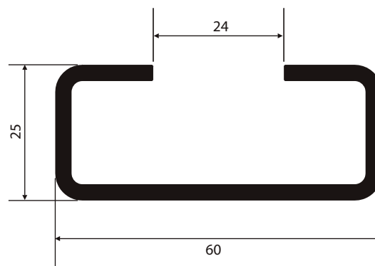
NI-646 1,040 Kg/m
